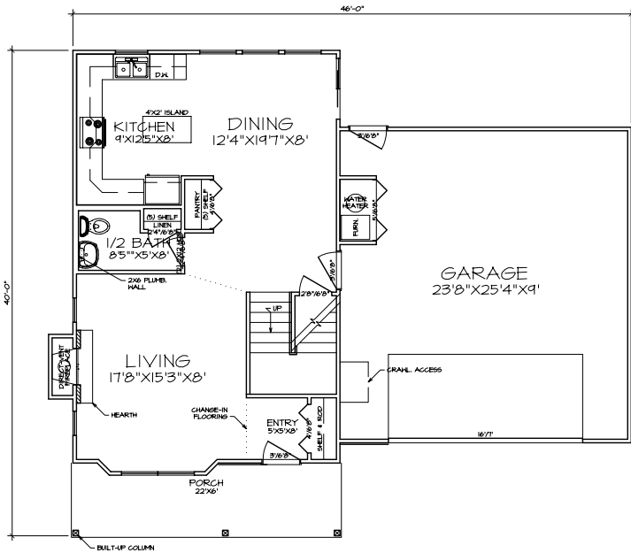
1 FIRST FLOOR PLAN A-4
